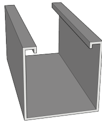
6" X 6" X .190" (6063-T6)
