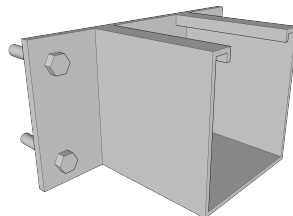
U-BEAM TO PLATE CONNECTION
